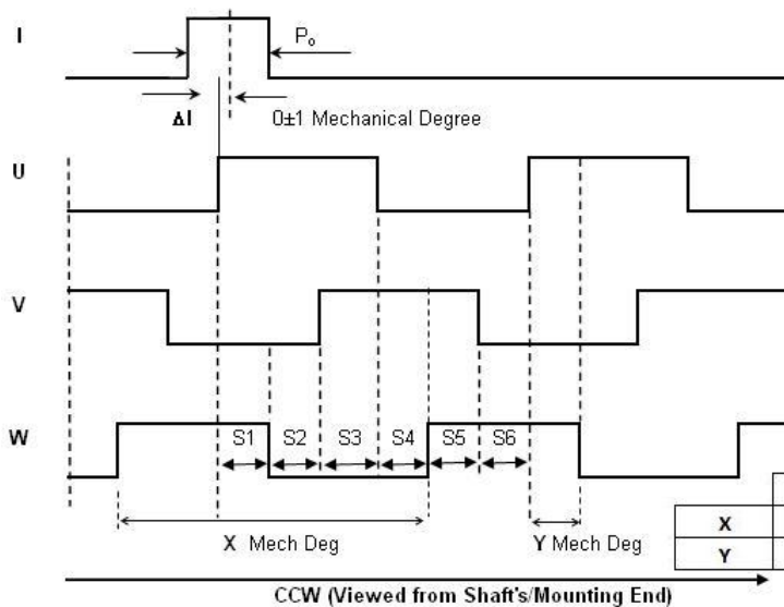
INDEX AND COMMUTATION SIGNALS
