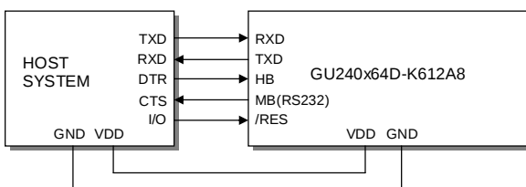
Asynchronous serial communication from host system to VFD module.
