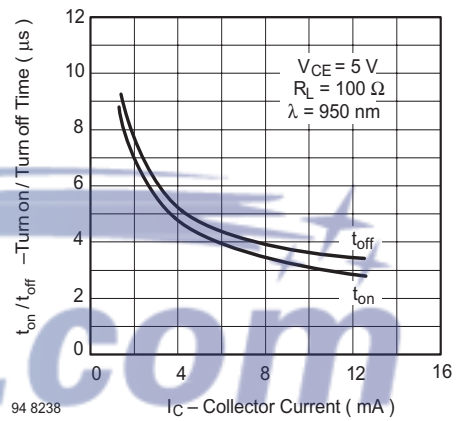
Figure 7. Turn On/Turn Off Time vs. Collector Current
