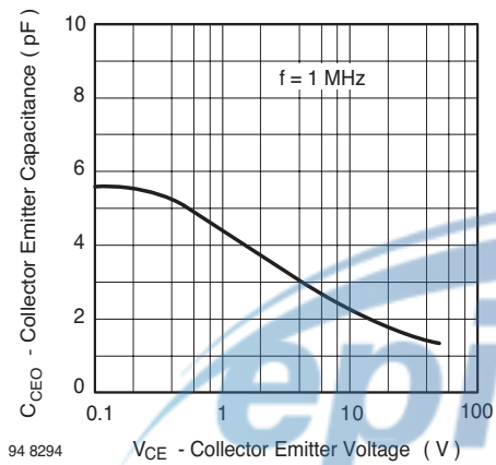
Figure 6. Collector Emitter Capacitance vs. Collector Emitter Voltage
