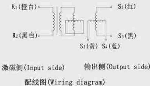
旋转变压器引线定义 (Resolver down-lead define)
