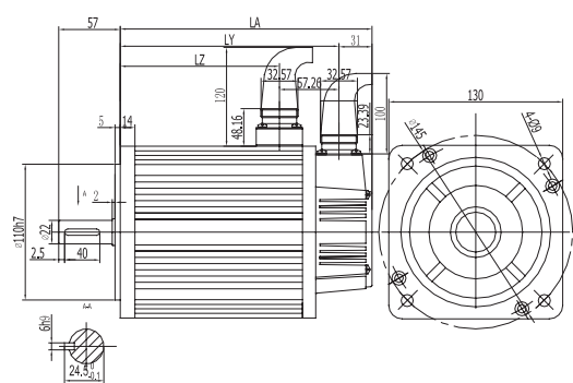
( 2 ) 380V 伺服电机尺寸
