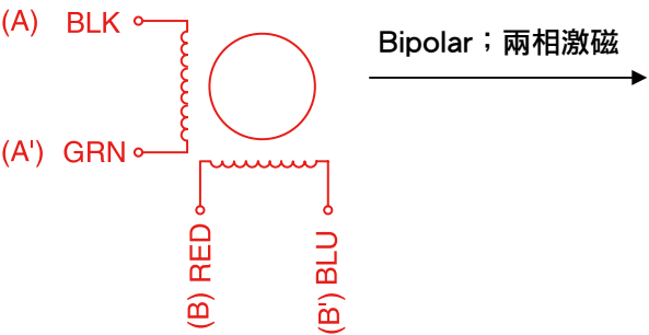
WIRING DIAGRAM
