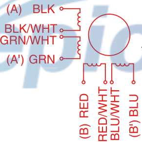
WIRING DIAGRAM
