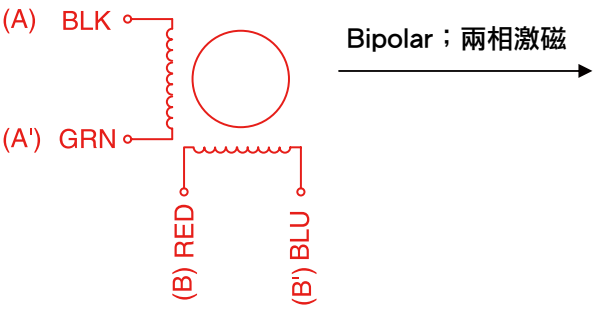
WIRING DIAGRAM
