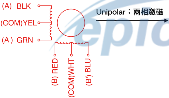
WIRING DIAGRAM
