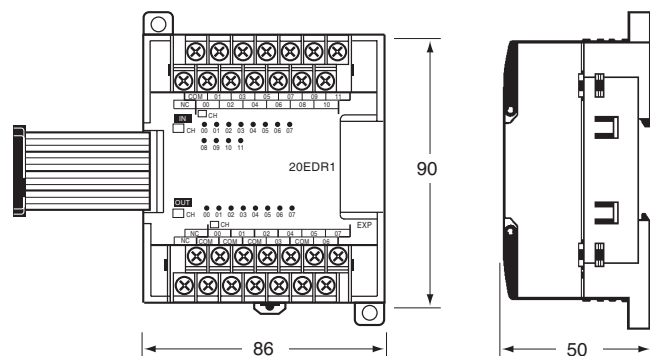
CPM1A-20ED □
