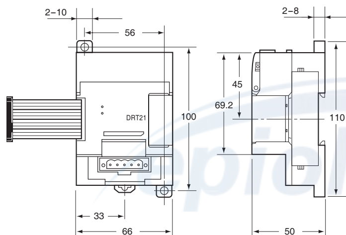
CPM1A-DRT21
