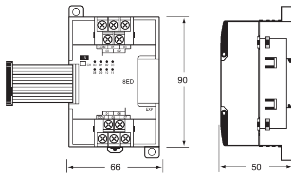
CPM1A-8 □ □ □
