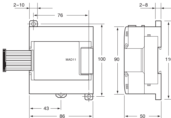
CPM1A-MAD11
