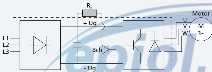
Connection diagram
