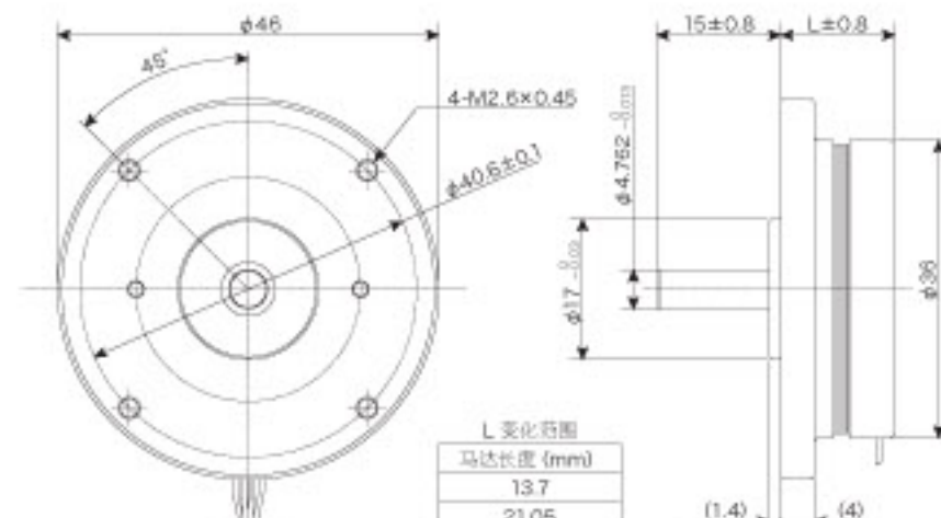
SST36CXXX3
