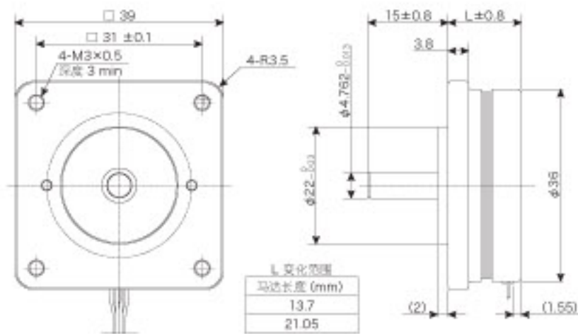
SST36CXXX2
