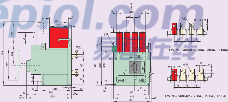
图16-1 DW17D-1900/4(In=630~1900)四极固定式水平接线
