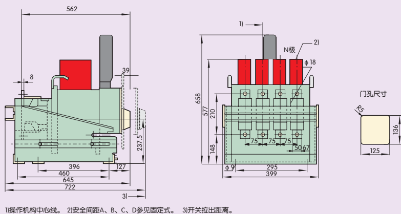
图16-5 DW17D-1900/4( I_n=630A\sim 1600A )四极抽屉式接线
