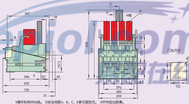
图16-6 DW17D-1900/4( I_n=1900A )四极抽屉式接线
